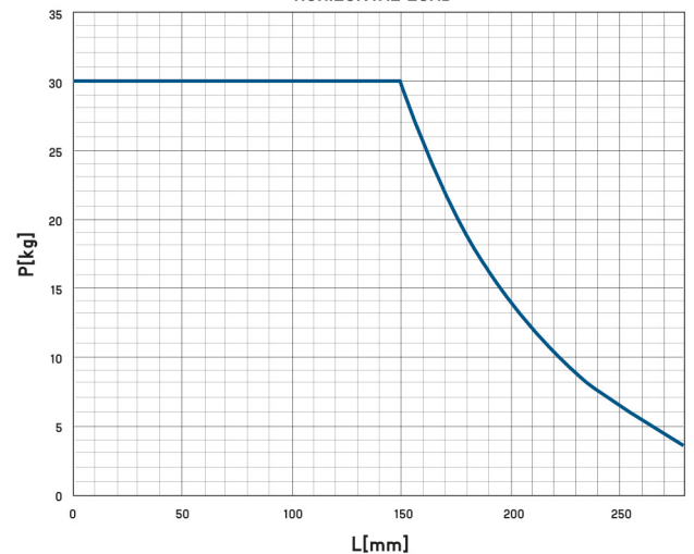
HORIZONTAL LOAD
