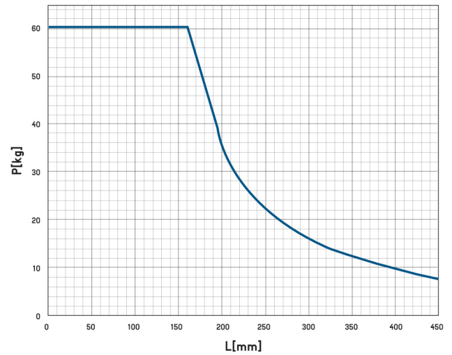
VERTICAL LOAD
